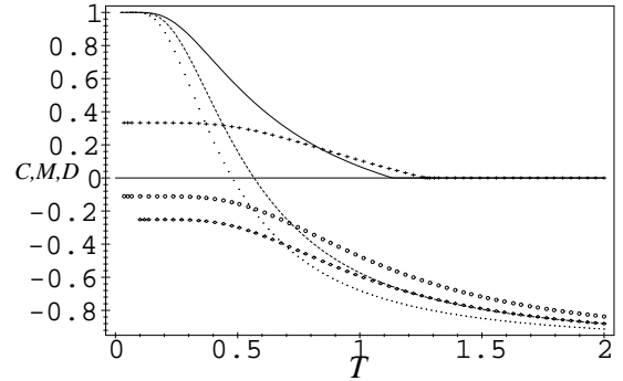
FIG. 4. The violation measure D of the disorder inequality, the concurrence C and violation measure M as a function of T . We plotted C (solid line), M (dashed line), and R (dotted line) for N = 2 and C (cross points), M (circle points), and R (diamond points) for N = 3 , respectively. The parameters J = -1 and B = \Delta = 0 .
